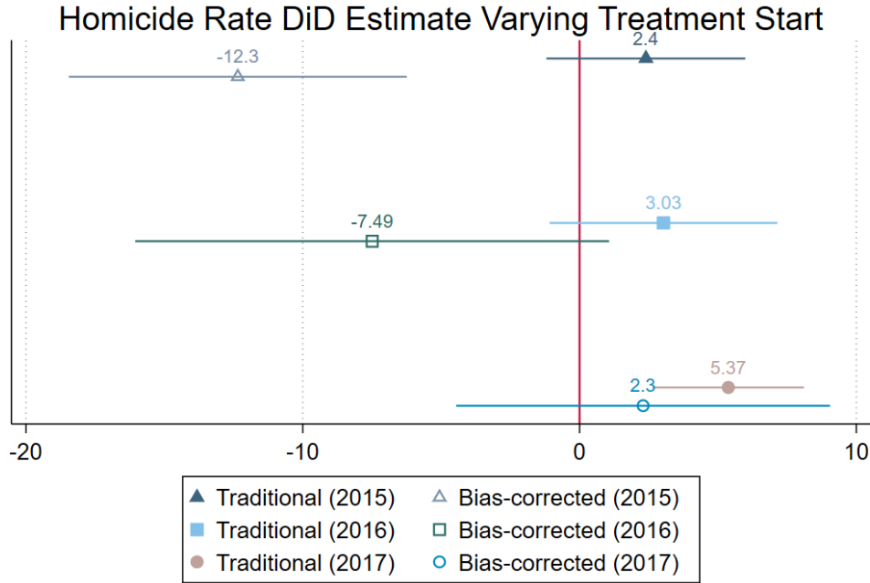
Figure 5: DiD estimate of average increase in homicide rate due to treatment, varying the treatment period from 2015 (top) to 2017 (bottom). Solid (hollow) markers represent results from traditional (bias-corrected) SCM.
